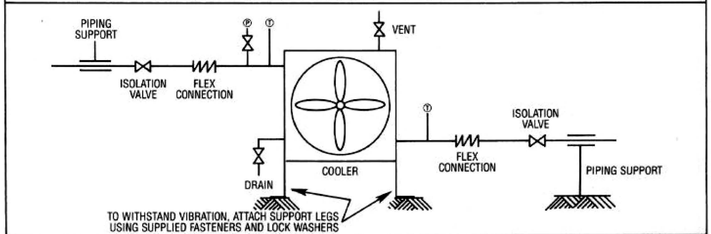
FIG. 2 SUGGESTED LIQUID COOLER INSTALLATION/FLOW DIAGRAM
