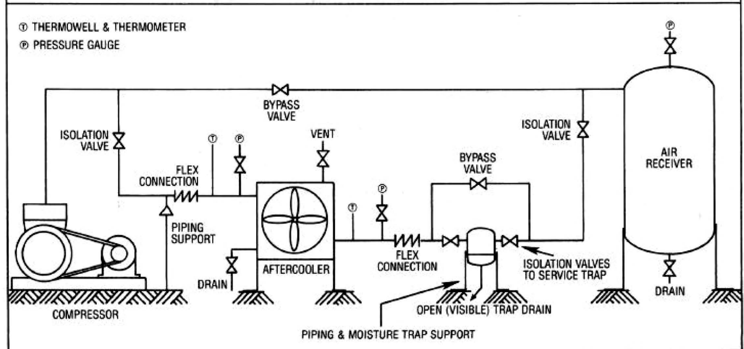
FIG. 3 SUGGESTED AFTERCOOLER INSTALLATION/FLOW DIAGRAM
