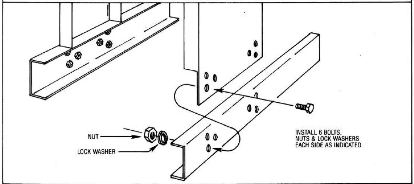
FIG. 1 LEG ASSEMBLY
