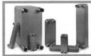
Brazed Plate Heat Exchangers
