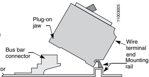
Figure 5: Homeline Branch Circuit Breaker
